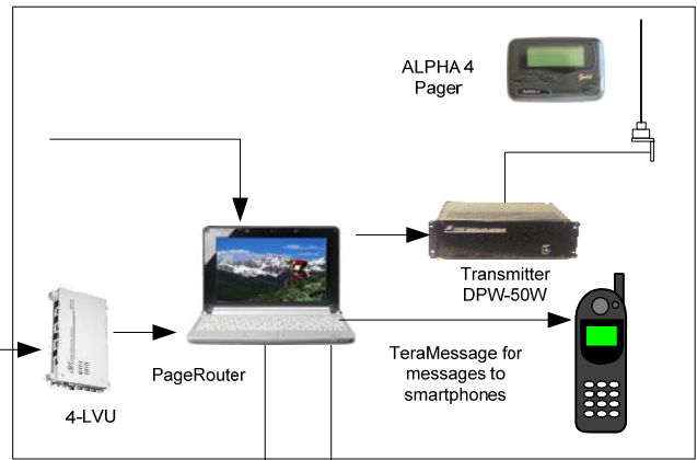
Antenna delivered with 50 ft. cable. Install antenna as high as possible for maximum paging range (1 to 10 miles depending on terrain and antenna height).
